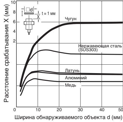
E2A-M12□N08/E2A-S12□N08
